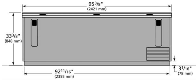
SPC: 870876 APN: 8344772 SPC: 871900 APN: 9380726 Front View
