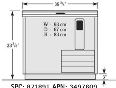
SPC: 871891 APN: 3497609 SPC: 021585 APN: 0089870 Front View
