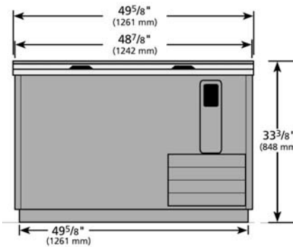
SPC: 870874 APN: 6344774 SPC: 021595 APN: 0089961 Front View
